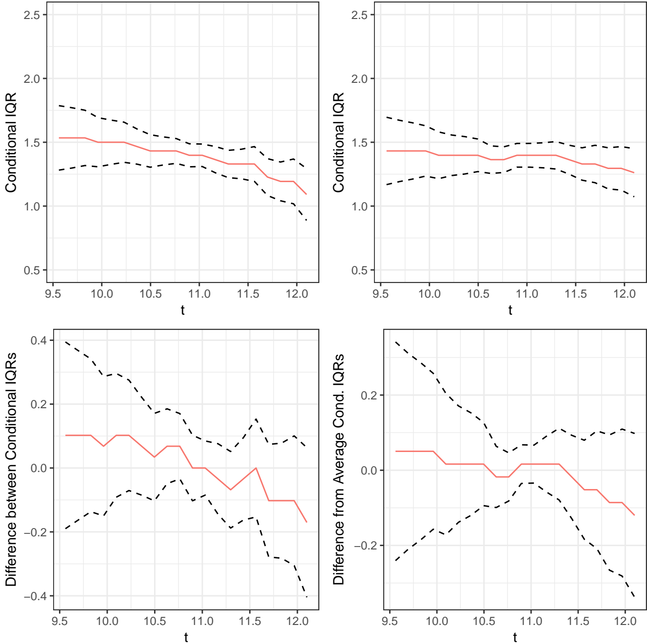
Figure 5: Inter-Quantile Ranges
